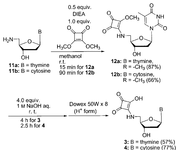
Scheme 3. Synthesis of deoxynucleoside 5'-phosphate analogues.
