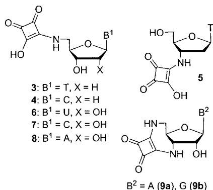
Scheme 2. Structures of squaramide-type nucleotide analogues.
