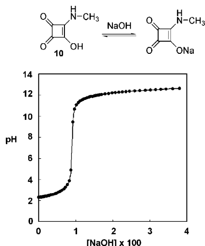
Figure 1. Alkaline titration of squaramide.
