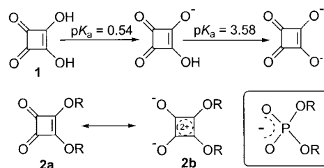
Scheme 1. Structures of squaric acid derivatives.
