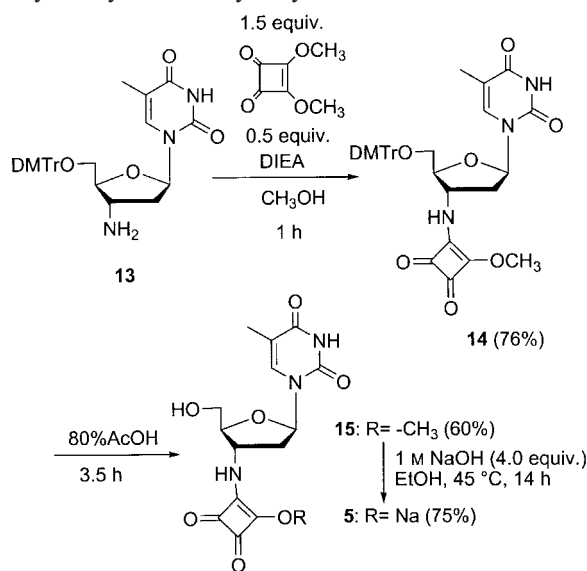
Scheme 4. Synthesis of thymidine 3'-phosphate analogues.
